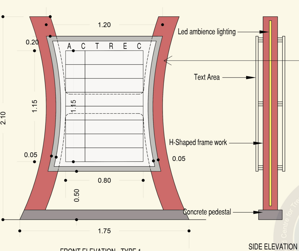
FRONT ELEVATION - TYPE 1
